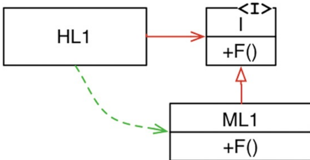
Figure 5.2 Dependency inversion
