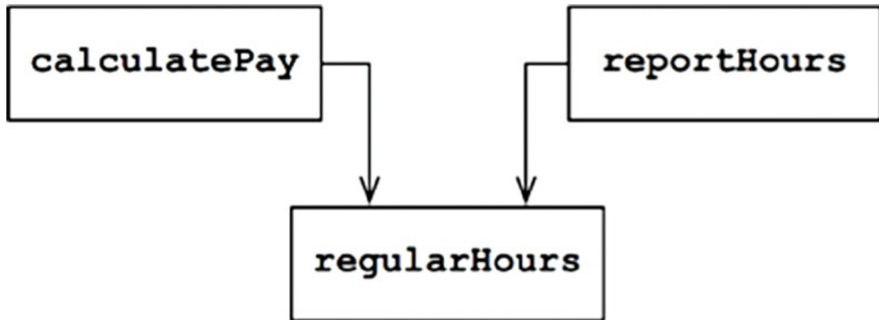
Figure 7.2 Shared algorithm
